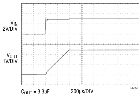
Figure 3. Start-Up Response
