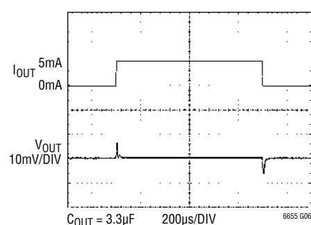
1.25V Sinking Current with a 3.3µF Output Capacitor
