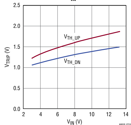
2.5V \overline{SHDN} Input Voltage Thresholds vs V_{IN}
