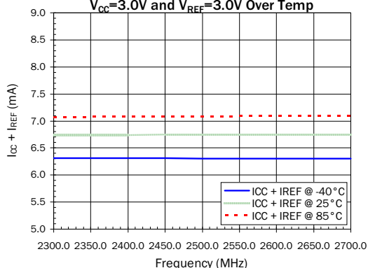
I_{CC} + I_{REF} at WiFi Band in High Gain Mode
