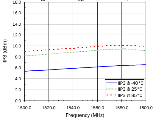
IIP3 @ GPS Band in Bypass Mode
