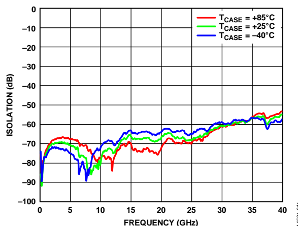
Figure 11. Isolation Between RF1 and RF2 vs. Frequency over Temperature
