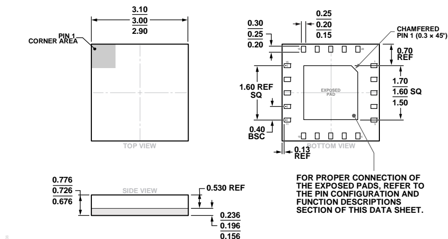
Figure 24. 20-Terminal Land Grid Array [LGA] 3 mm × 3 mm Body and 0.72 mm Package Height (CC-20-3) Dimensions shown in millimeters
