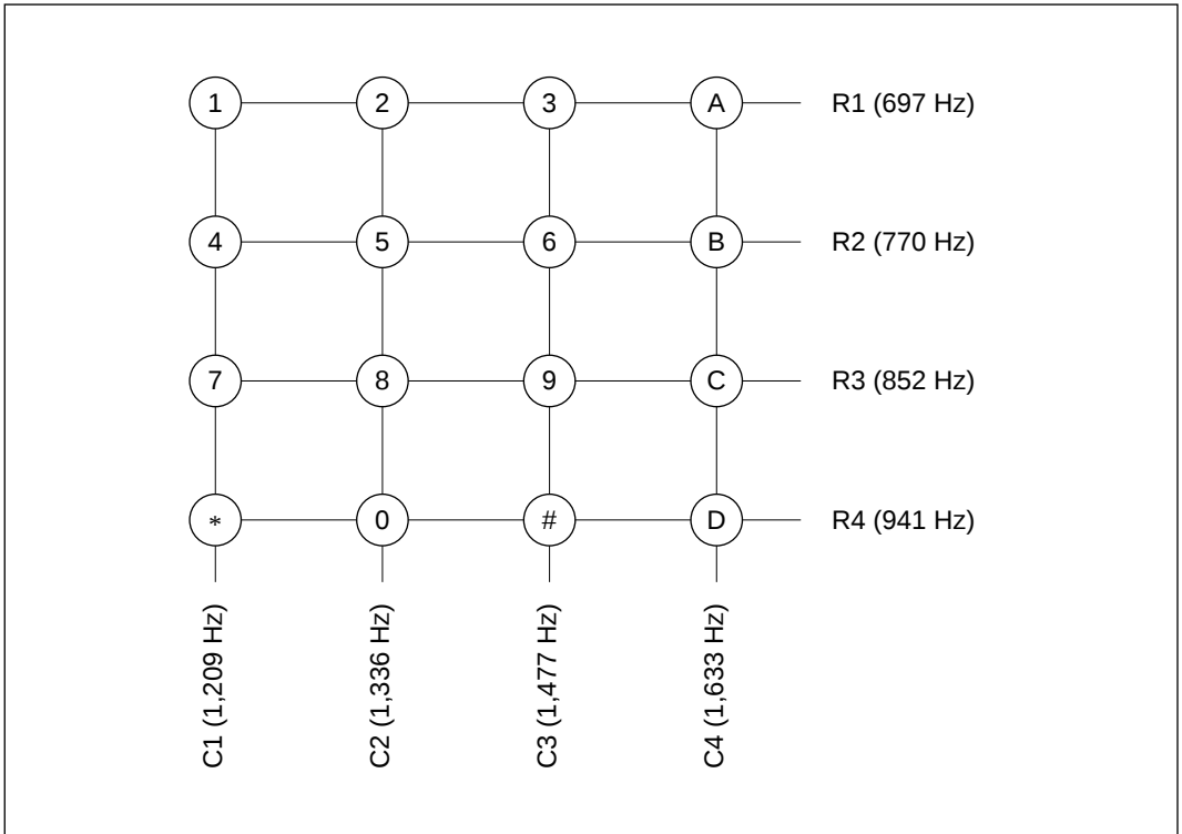
Figure 11-1 DTMF Frequencies
