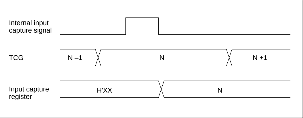
Figure 9-4-6 Input Capture Timing
