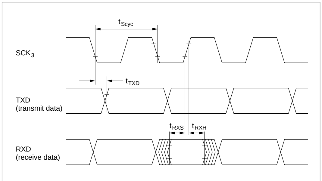
Figure 15-9 Input/Output Timing of Serial Interface 3 in Synchronous Mode
