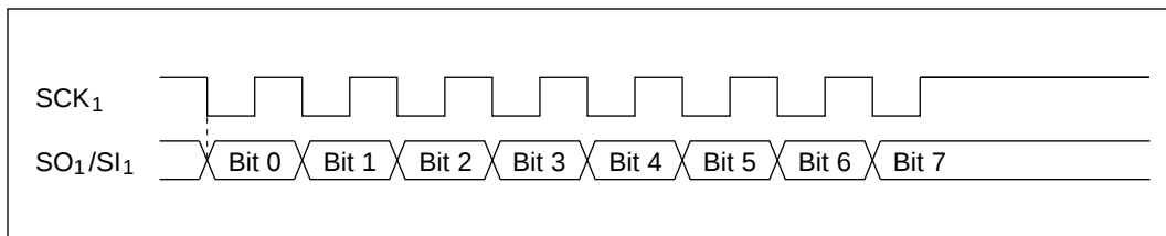
Figure 10-2-2 Transfer Format
