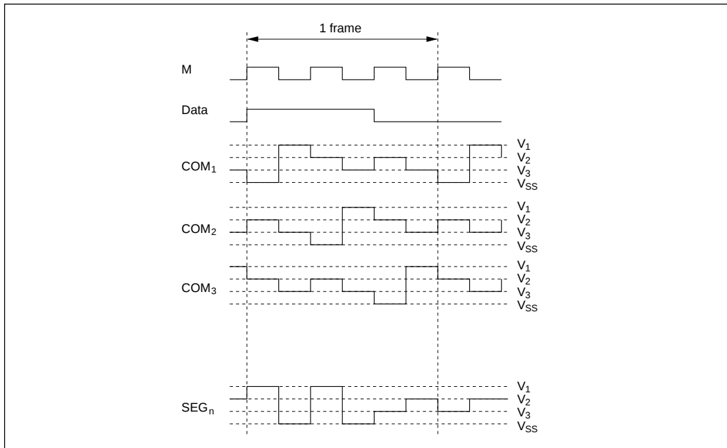
Figure 13-11 (b) Waveforms at 1/3 Duty
