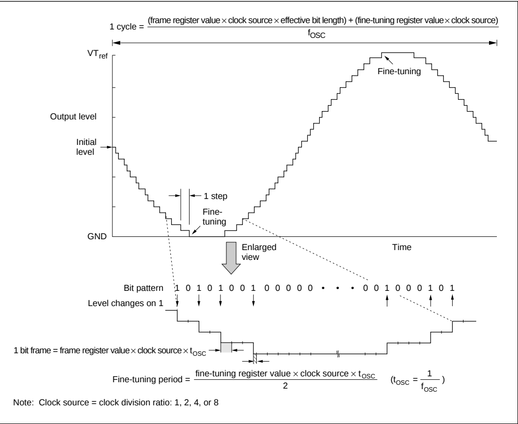
Figure 14-2 Multitone Generator Output Waveform
