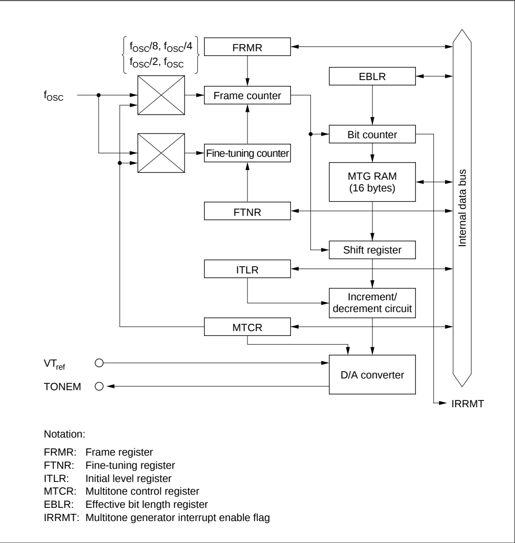
Figure 14-1 Multitone Generator Block Diagram
