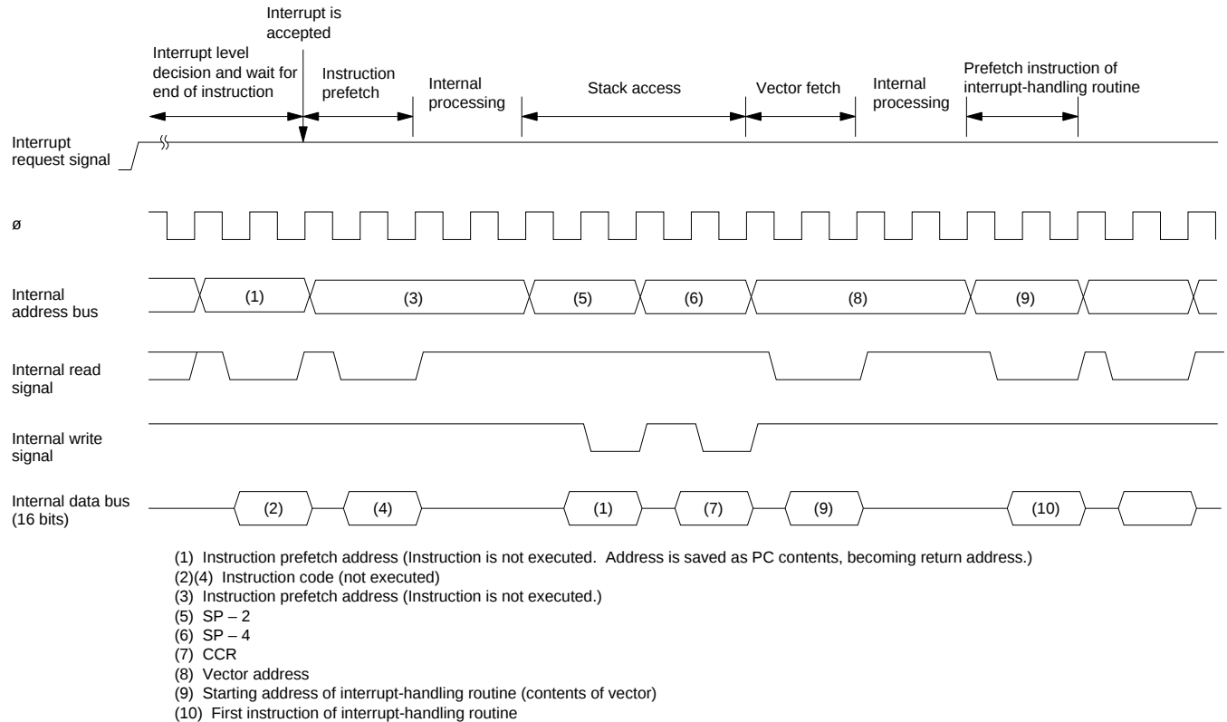
Figure 3-5 Interrupt Sequence
