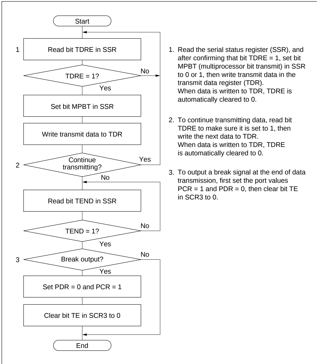
Figure 10-3-17 Typical Multiprocessor Data Transmission Flow Chart
