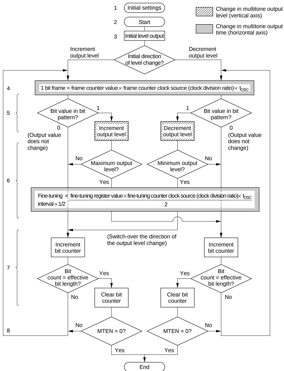
Figure 14-3 Flow Chart of Multitone Generator Operation
