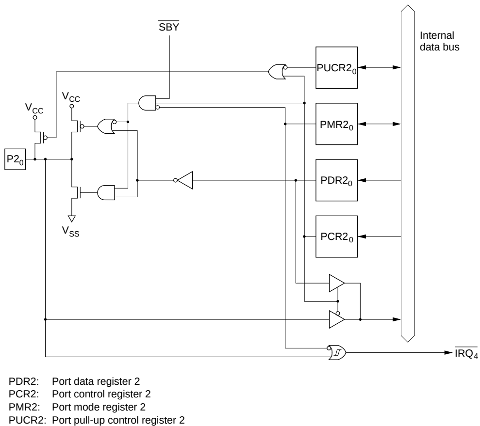
Figure C-2 (h) Port 2 Block Diagram (Pin P2 0 )
