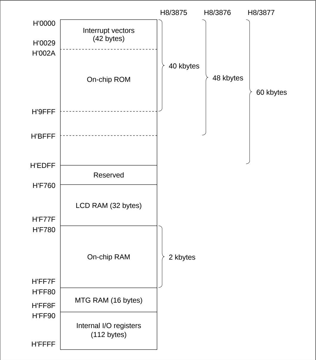
Figure 2-16 H8/3877 Series Memory Map
