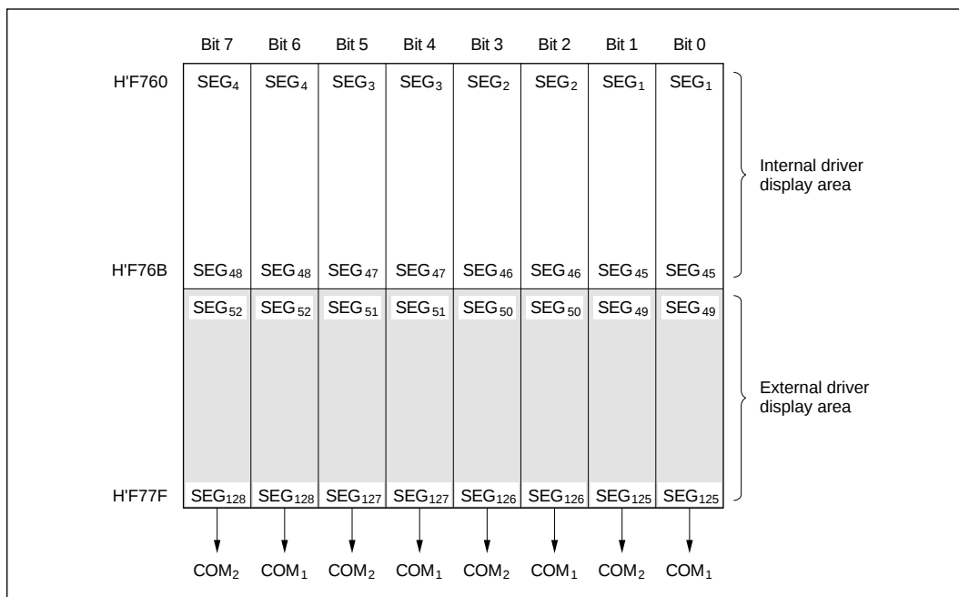
Figure 13-7 LCD RAM Map 1: External Segment Expansion (1/2 Duty)
