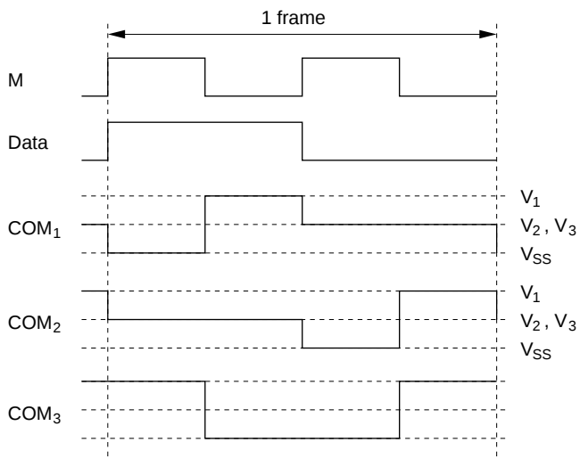
Figure 13-11 (c) Waveforms at 1/2 Duty
