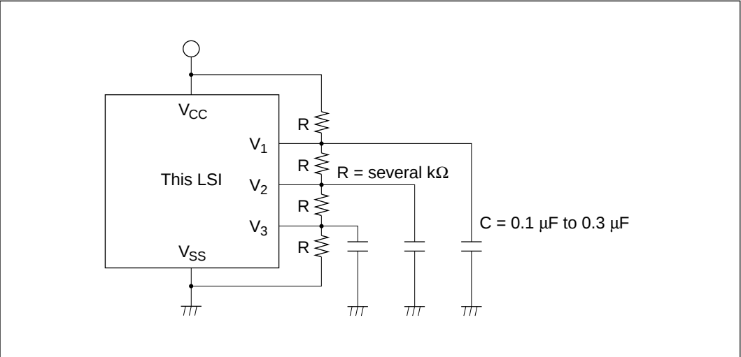
Figure 13-12 Connecting an External Resistive Voltage Divider
