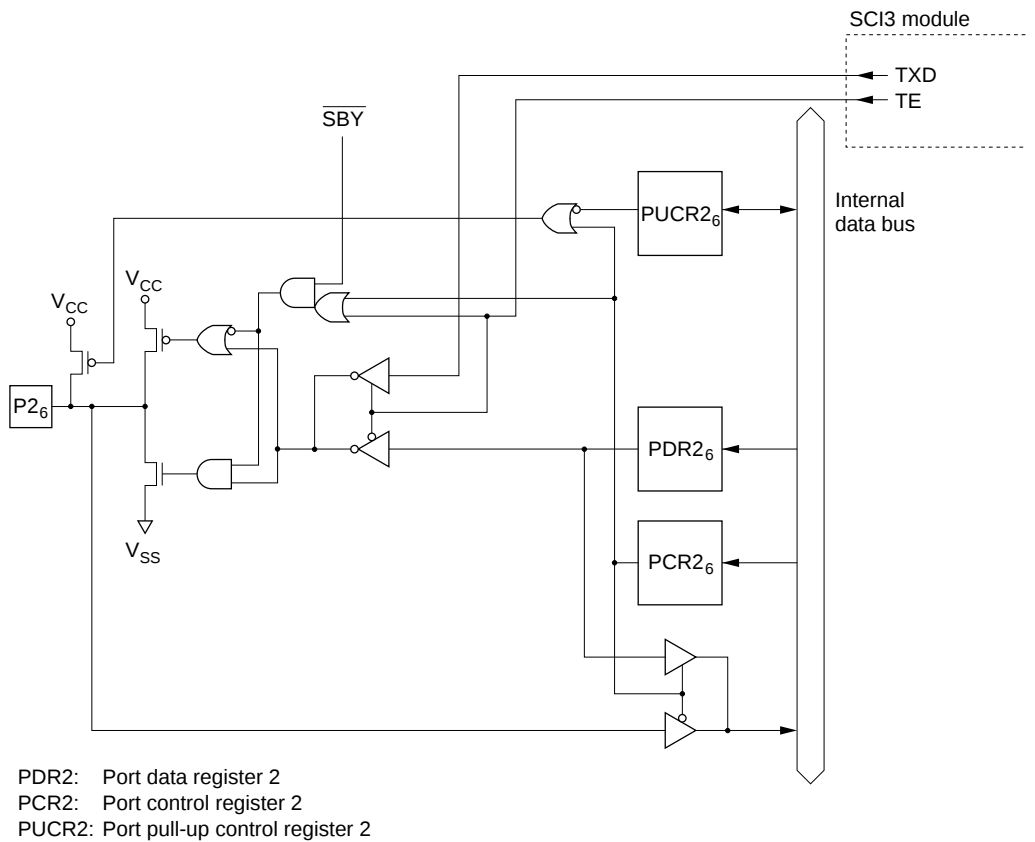
Figure C-2 (b) Port 2 Block Diagram (Pin P2 6 )
