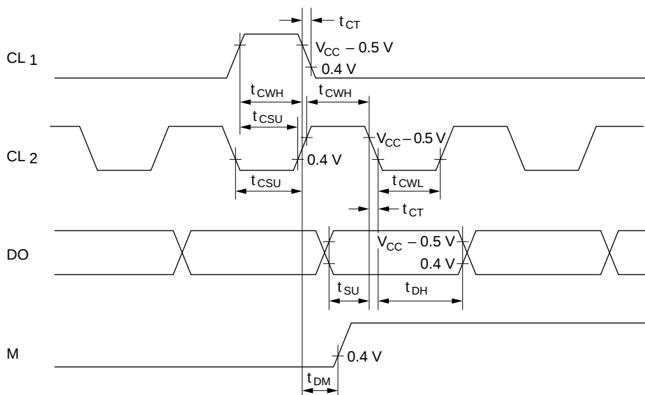
Figure 15-1 Segment Expansion Signal Timing
