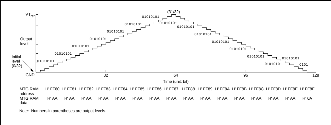
Figure 14-6 Typical Bit Pattern for Triangle Wave
