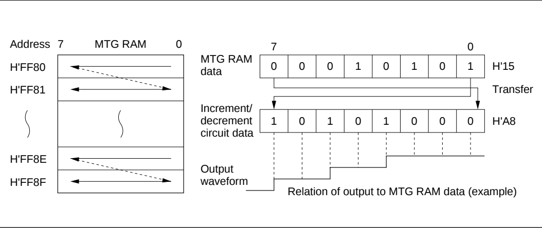
Figure 14-4 Bit Pattern on MTG RAM
