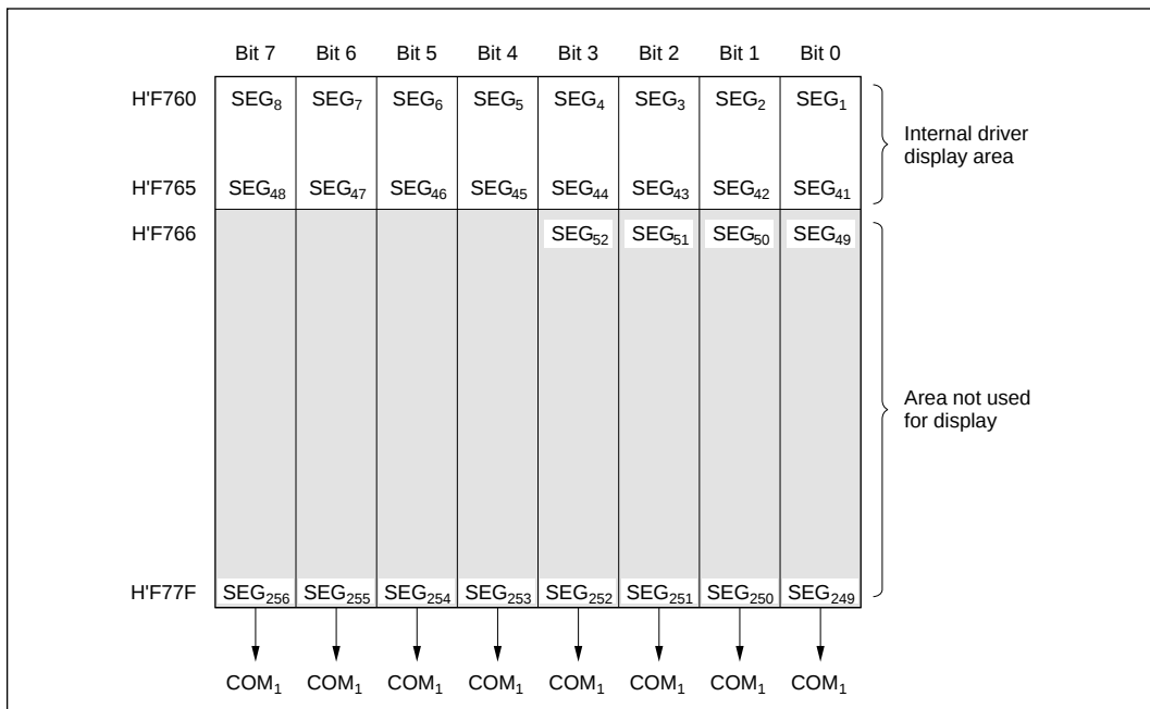
Figure 13-8 LCD RAM Map 2: External Segment Expansion (Static Duty)
