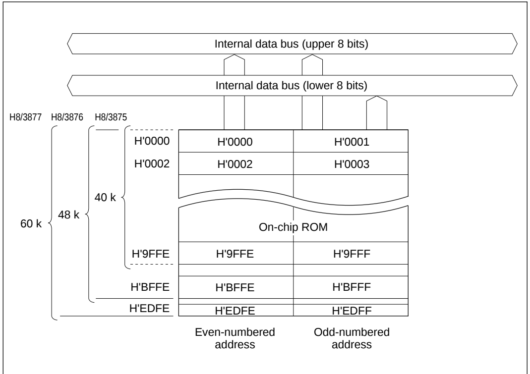
Figure 6-1 ROM Block Diagram
