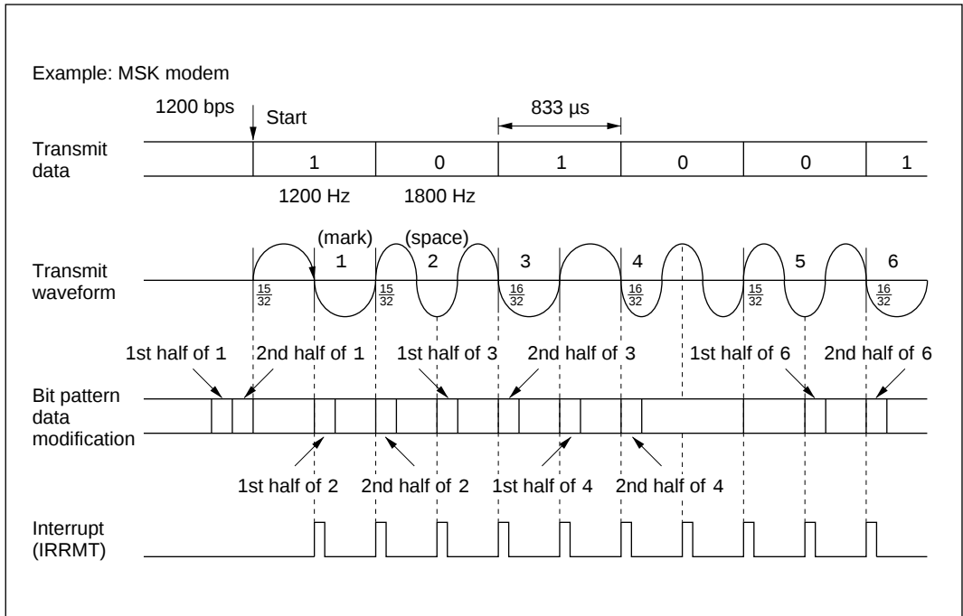
Figure 14-8 Timing of Interrupts and Bit Pattern Data Modification
