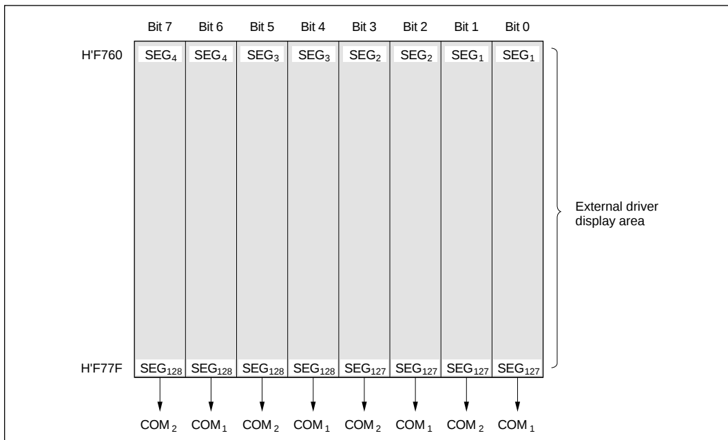
Figure 13-9 LCD RAM Map When All External Segments are Used (Example: SGX = 1, SGS3 to SGS0 = 0000, 1/2 Duty)
