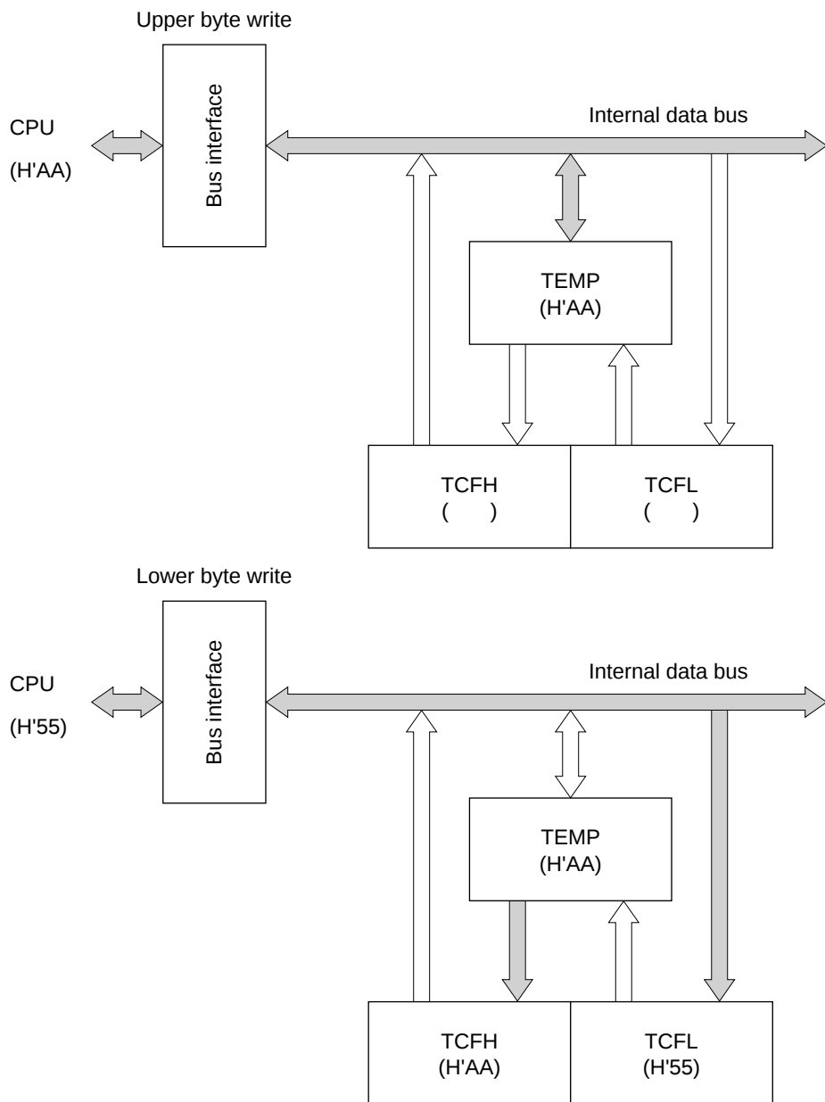
Figure 9-3-2 TCF Write Operation (CPU → TCF)
