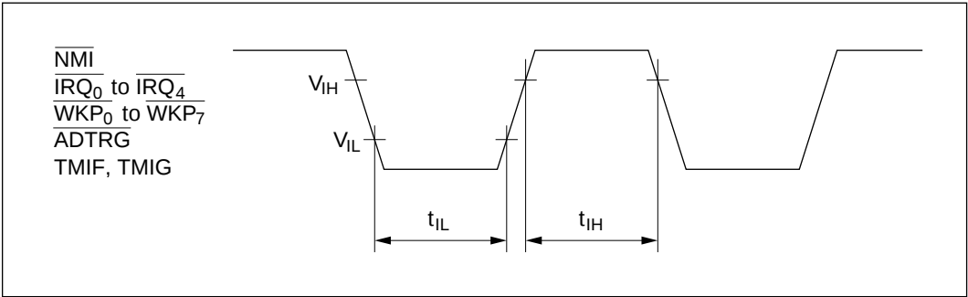
Figure 15-6 Input Timing
