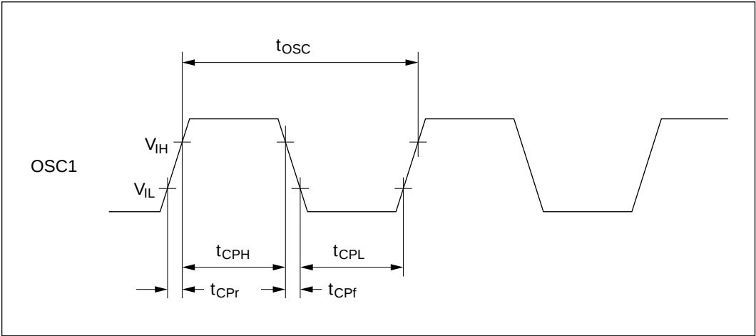
Figure 15-4 System Clock Input Timing
