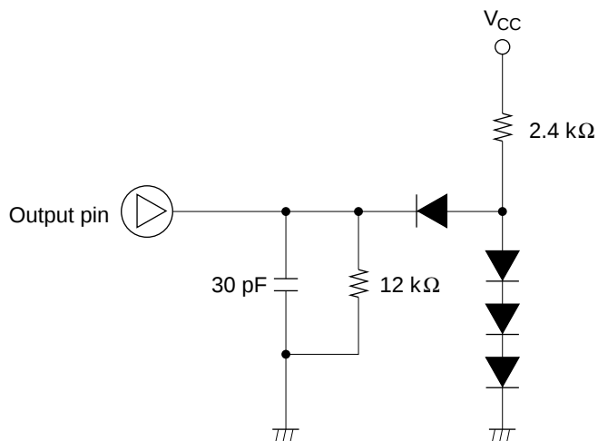
Figure 15-10 Output Load Condition
