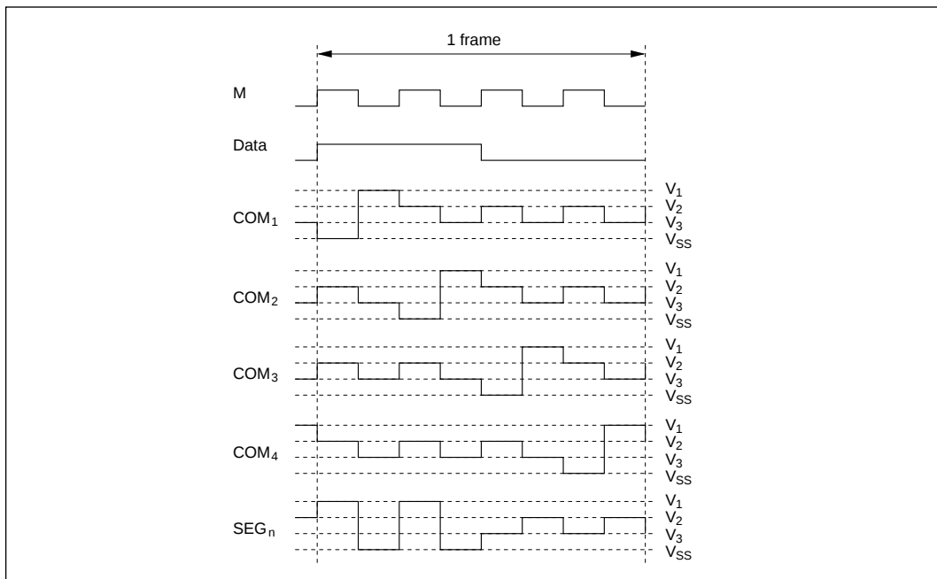
Figure 13-11 (a) Waveforms at 1/4 Duty
