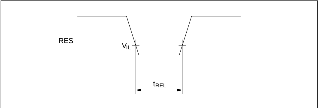
Figure 15-5 \overline{RES} Low Width
