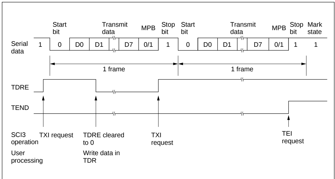
Figure 10-3-18 Typical Multiprocessor Format Transmit Operation (8-Bit Data, Multiprocessor Bit Added, and 1 Stop Bit)
