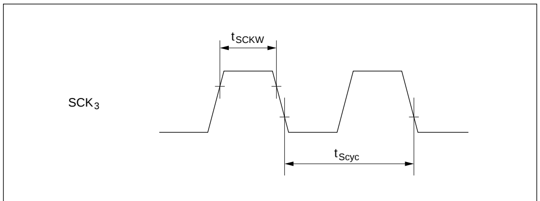
Figure 15-8 SCK 3 Input Clock Timing
