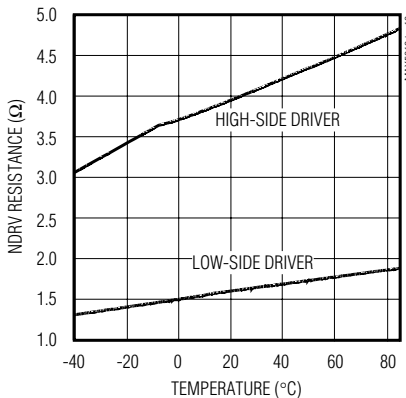
NRDV RESISTANCE vs. TEMPERATURE
