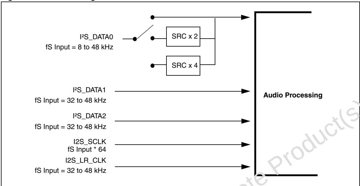
Figure 21. I 2 S block diagram
