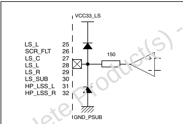
Figure 34. VCC33_LS
