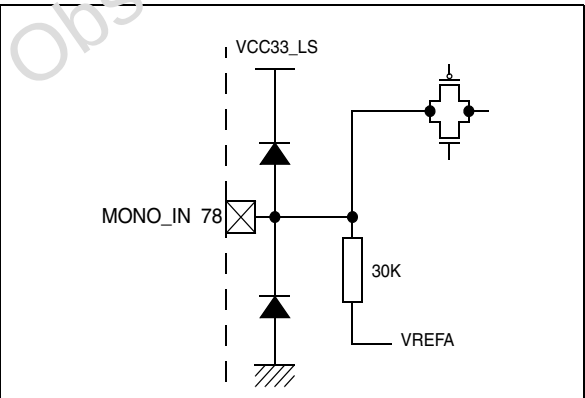
Figure 35. MONO_IN
