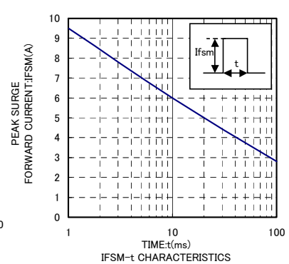
TIME:t(ms) IFSM-t CHARACTERISTICS
