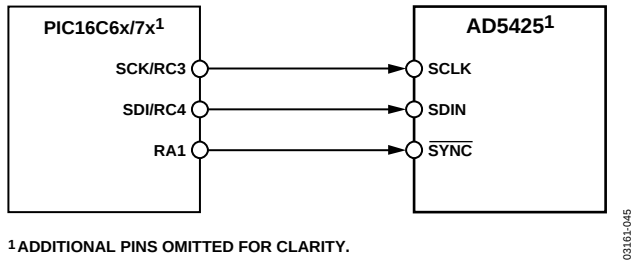
Figure 45. PIC16C6x/7x-to-AD5425 Interface
