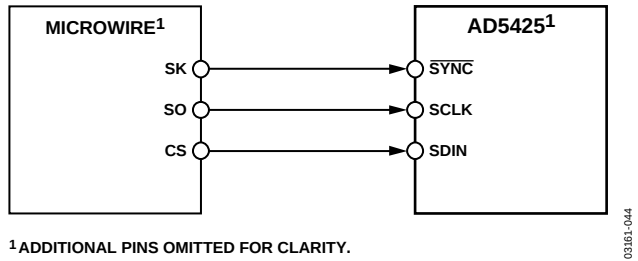
Figure 44. MICROWIRE-to-AD5425 Interface
