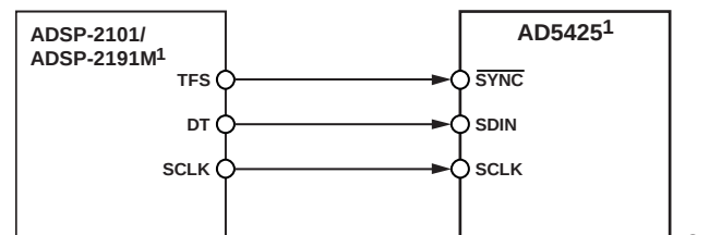
Figure 39. ADSP-2101/ADSP-2191M SPORT-to-AD5425 Interface
