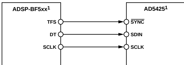
Figure 41. ADSP-BF5xx-to-AD5425 Interface
