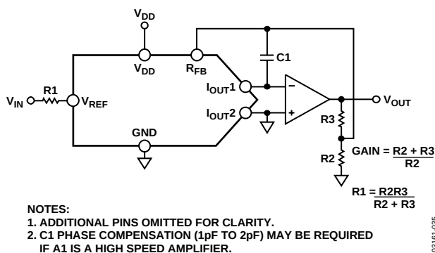
Figure 35. Increasing the Gain of Current Output DAC
