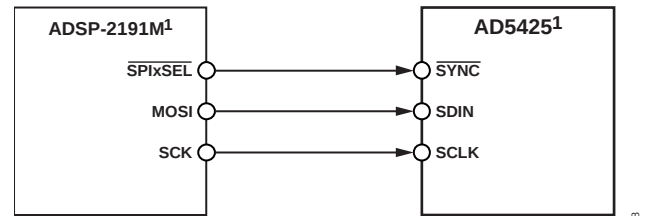
Figure 38. ADSP-2191M SPI-to-AD5425 Interface
