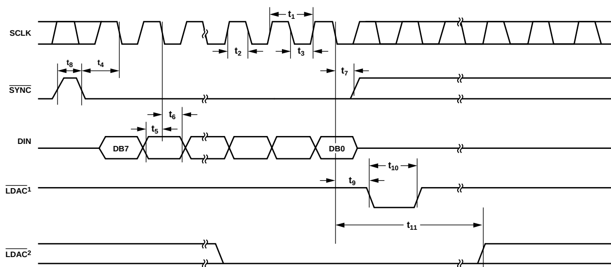
Figure 2. Timing Diagram
