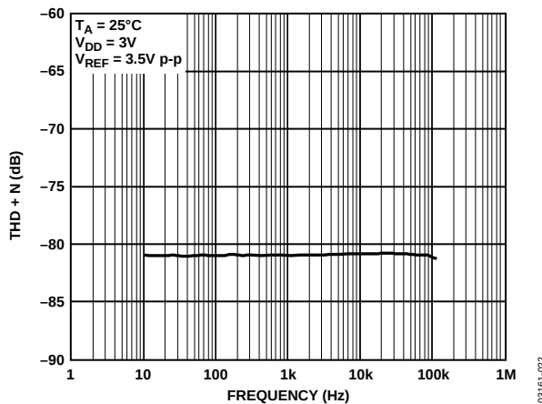
Figure 22. THD and Noise vs. Frequency
