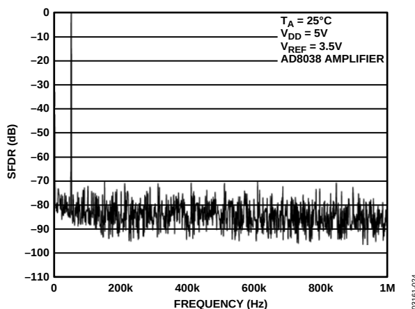
Figure 24. Wideband SFDR, Clock = 2 MHz, f_{OUT} = 50\text{ kHz}
