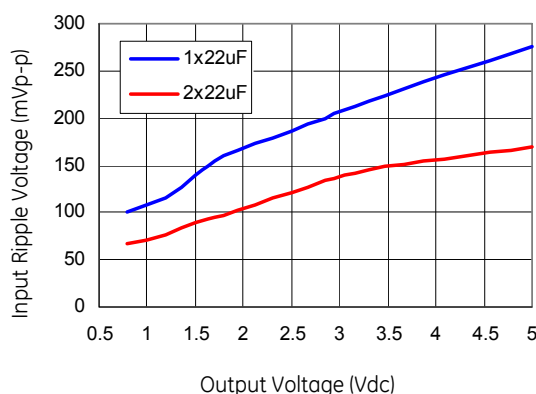
Figure 40. Input ripple voltage for various output voltages with 1x22 µF or 2x22 µF ceramic capacitors at the input (12A load). Input voltage is 12V.
