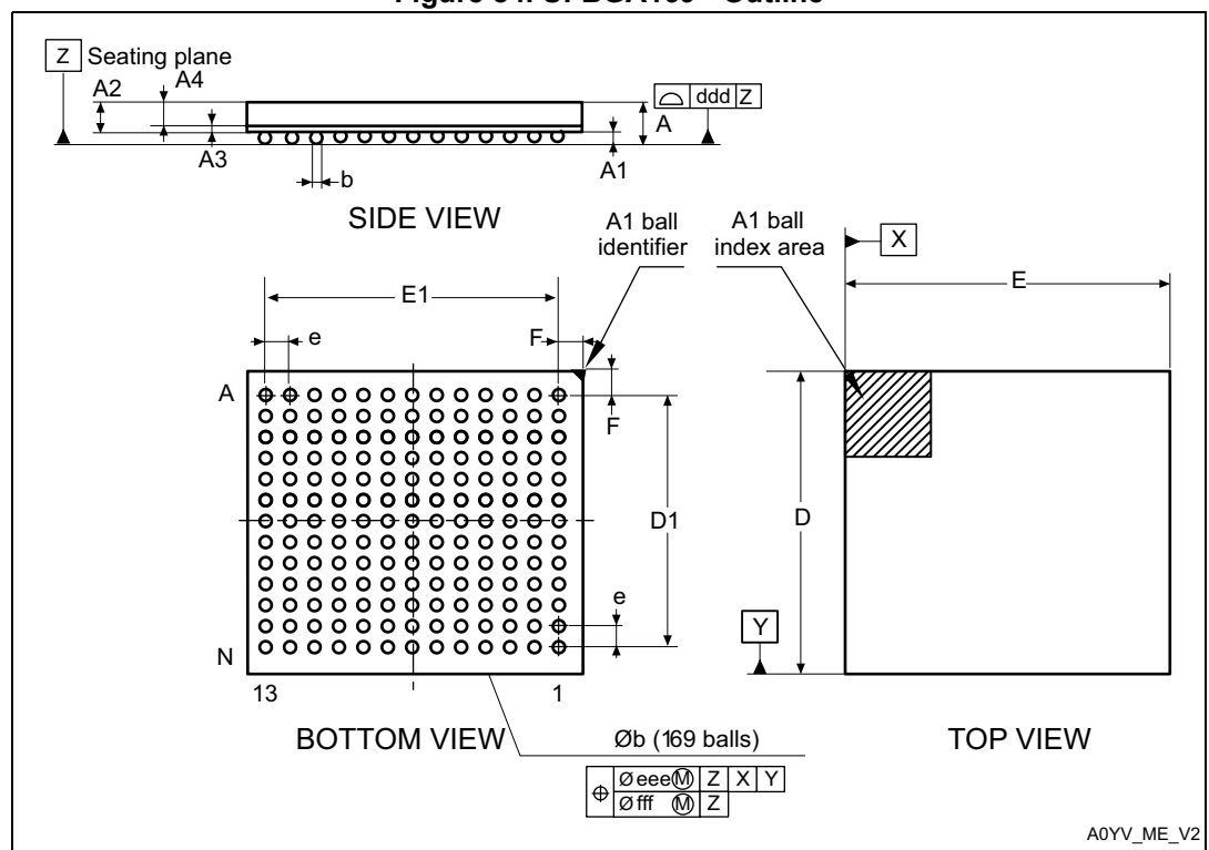
Figure 84. UFBGA169 - Outline
