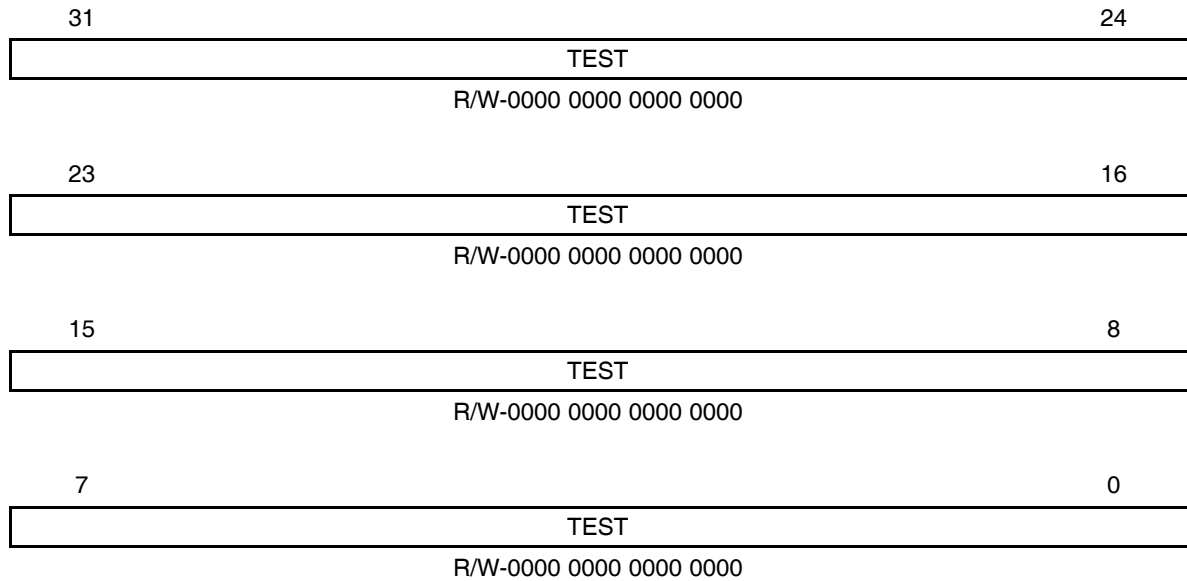
Figure 23. Test Register
