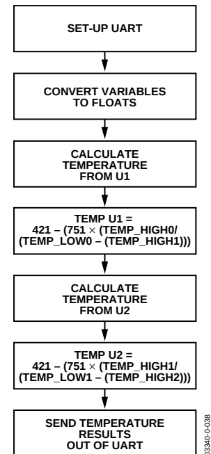
Figure 35. ADuC812 Temperature Calculation Routine Flowchart
