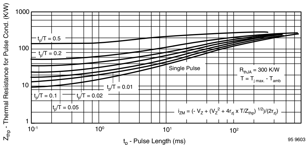
Fig. 10 - Thermal Response
