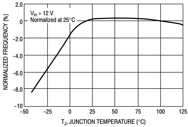
Figure 10. Oscillator Frequency
