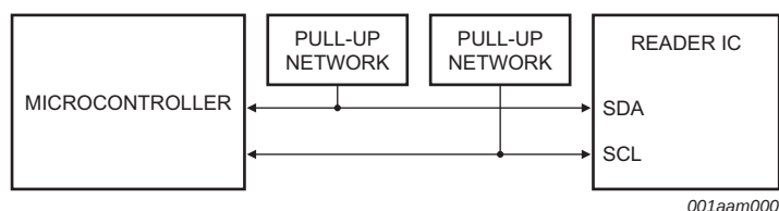
Fig 13. I 2 C-bus interface
