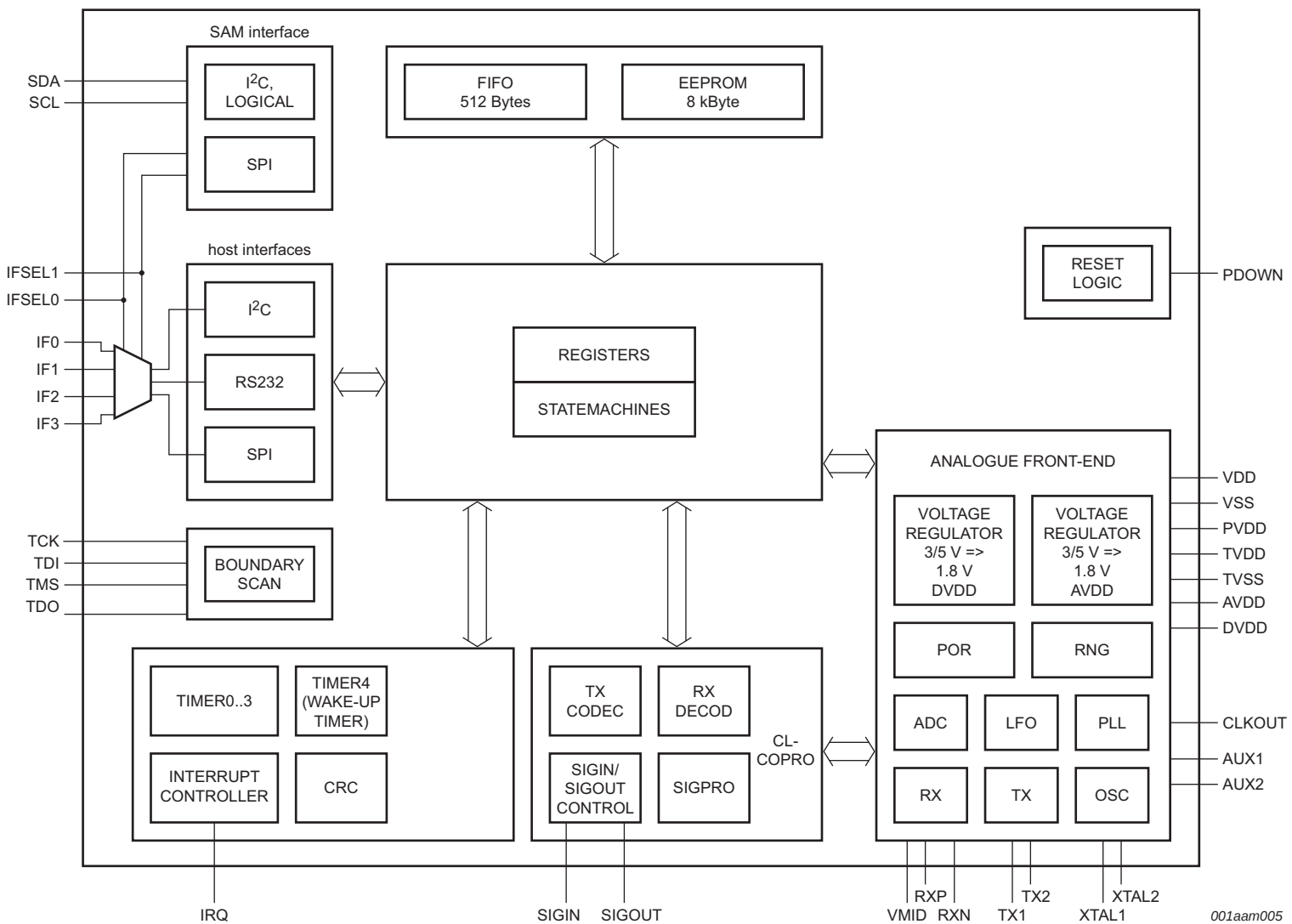
Fig 3. Detailed block diagram of the MFRC631
