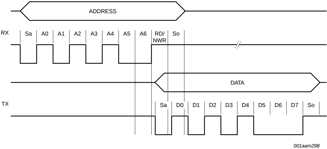
Fig 11. Example for UART Read
