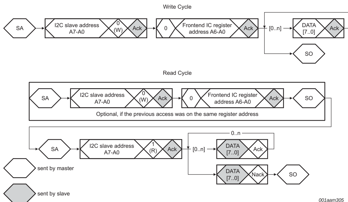
Fig 19. Register read and write access
