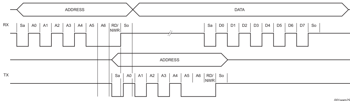
Fig 12. Example diagram for a UART write
