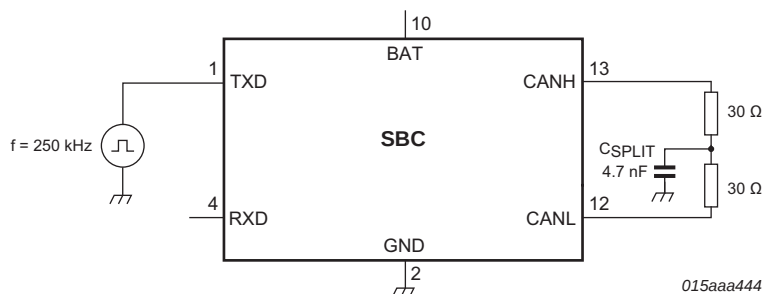
Fig 14. Test circuit for measuring transceiver driver symmetry
