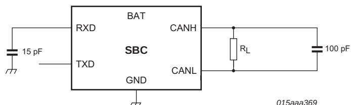
Fig 13. Timing test circuit for CAN transceiver
