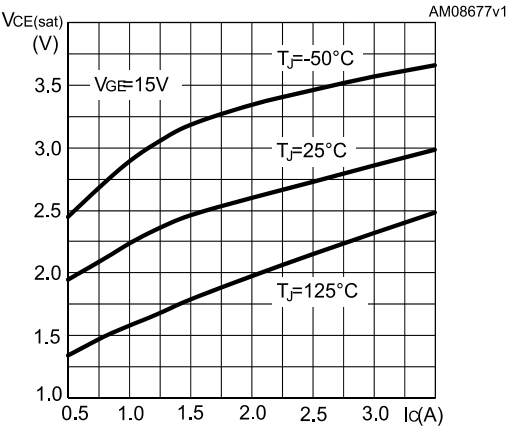
Figure 5: Collector-emitter on voltage vs collector current
