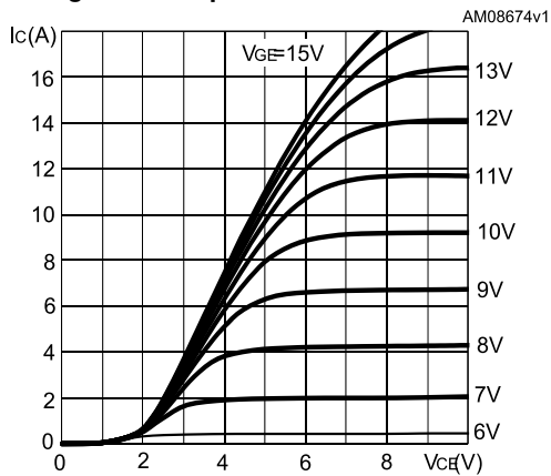
Figure 2: Output characteristics
