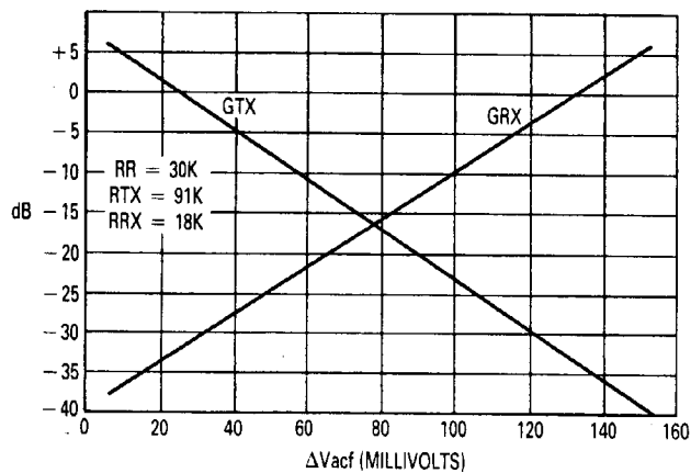
FIGURE 6 — ATTENUATOR GAIN versus \Delta V_{acf}
