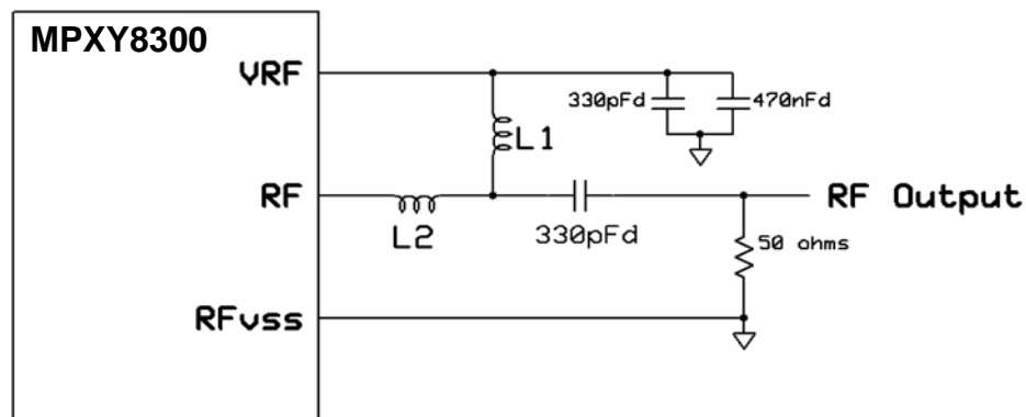
Output Power Measurement Configuration
