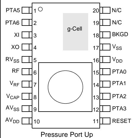
Figure 1. Pin Connections
