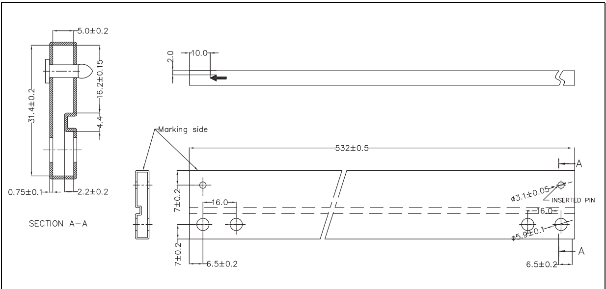
Figure 20. TO-220 single gauge tube outline(dimensions in mm)
