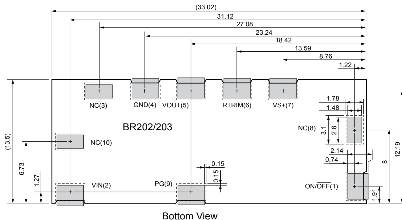
PCB Board Layout and Pin-out Diagram
