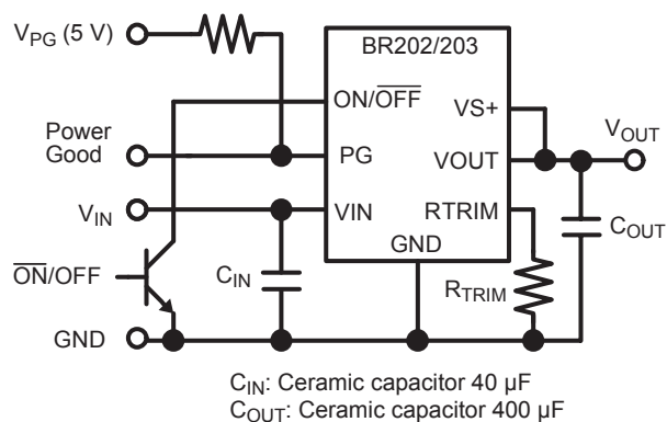
Figure 7. Test circuit for electrical characteristics
