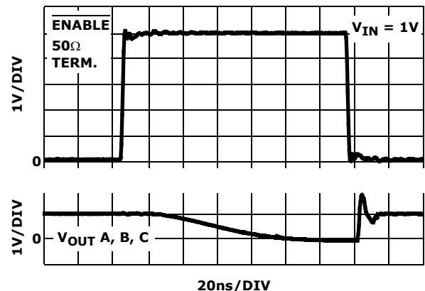
FIGURE 14. \overline{ENABLE} TRANSIENT RESPONSE V_{IN} = 1V
