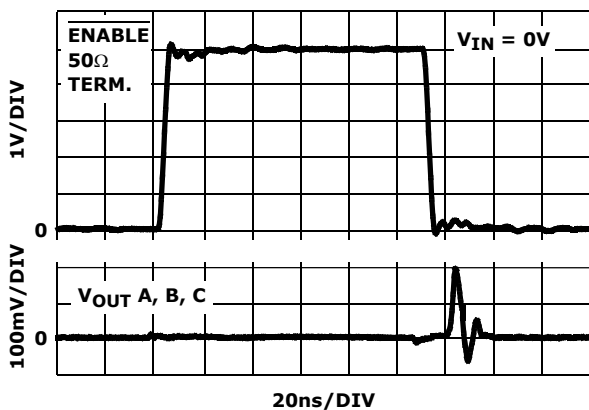
FIGURE 13. \overline{ENABLE} SWITCHING GLITCH V_{IN} = 0V
