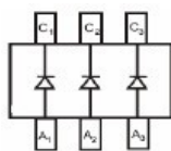
BAT54T
