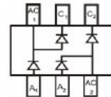
BAT54BR
