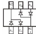
BAT54SD
