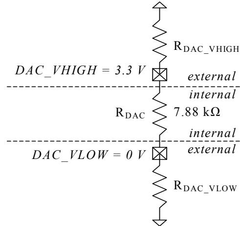
Figure 11: In- and external DAC connections
