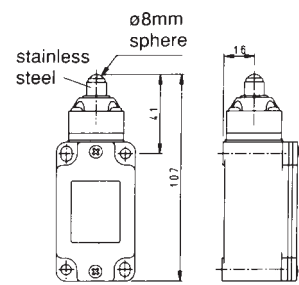
Actuator type 18 Rolling ball piston plunger
