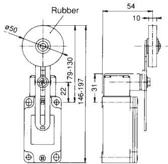
FD538 or FD5385 or FD938 + L353 FP538 or FP938 + L353 Turret type 38 Lever type L353 (single adjustment roller)
