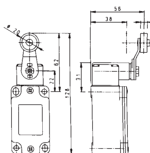
Actuator type 31 Roller-lever with small offset
