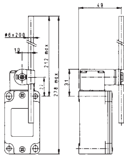
Actuator type 36 Adjustable glass-fibre rod lever
