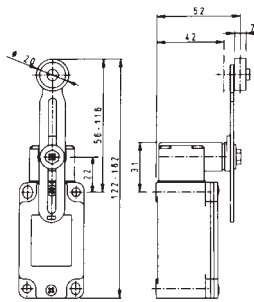
Actuator type 35 Adjustable roller lever
