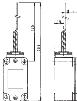
Actuator type 21 Sealed coil spring with cat's whisker
