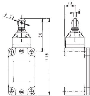
Actuator type 15 Sealed roller piston plunger
