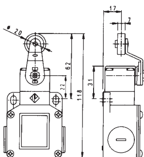
OF 920gcm PT 30° OT 45° MD 14° OP – OS 1.5m/s using a 30° cam Notes: 1. ø20mm plastic roller as standard, ø20mm metal roller actuator part no.: 511. 2. Lever position adjustable over 360° in 10° increments
