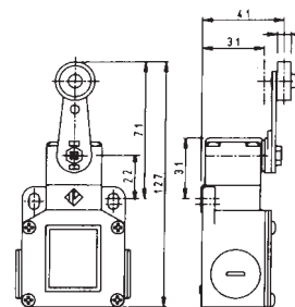
Notes: 1. \varnothing 20\text{mm} plastic roller as standard, \varnothing 20\text{mm} metal roller actuator part no.: 521; \varnothing 35\text{mm} plastic roller actuator part no.: 522; \varnothing 50\text{mm} rubber roller actuator part no.: 523. 2. Lever position adjustable over 360^\circ in 10^\circ increments
