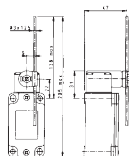
Actuator type 32 Adjustable round steel rod lever Actuator type 33 Adjustable square steel rod lever (rod 3x3x125)
