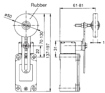
FD538 or FD5385 or FD938 + L354 FP538 or FP938 + L354 Turret type 38 Lever type L354 (dual adjustment roller)
