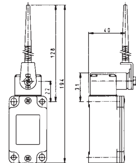
Actuator type 38+L34 Coiled spring lever with flexible rod
