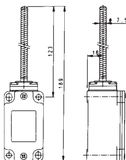
Actuator type 25 Sealed coil spring
