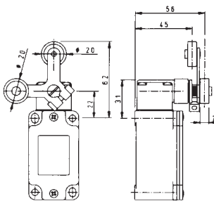
Actuator type 40 Dual roller lever with two stable free positions
