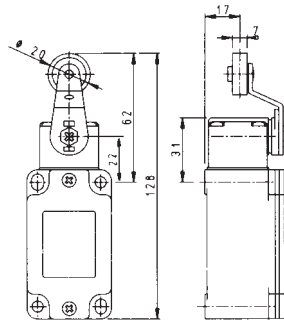
Actuator type 51 Roller-lever with large offset
