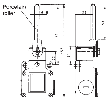
OF 615gcm PT 30° OT 45° MD 14° OP — OS — Note: Lever position adjustable over 360° in 10° increments
