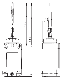
Actuator type 20 Sealed coil spring with flexible rod
