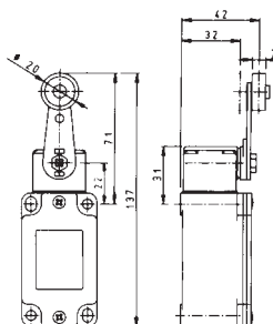
Actuator type 52 Roller lever without offset
