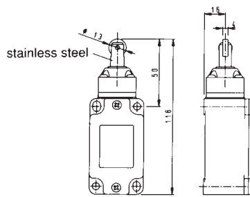
Actuator type 16 Roller piston plunger
