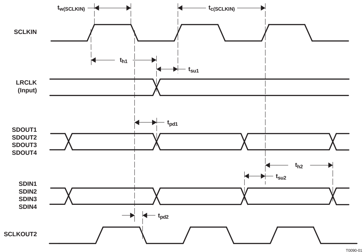
Figure 11-4. Serial Audio Port Slave Mode Timing Waveforms
