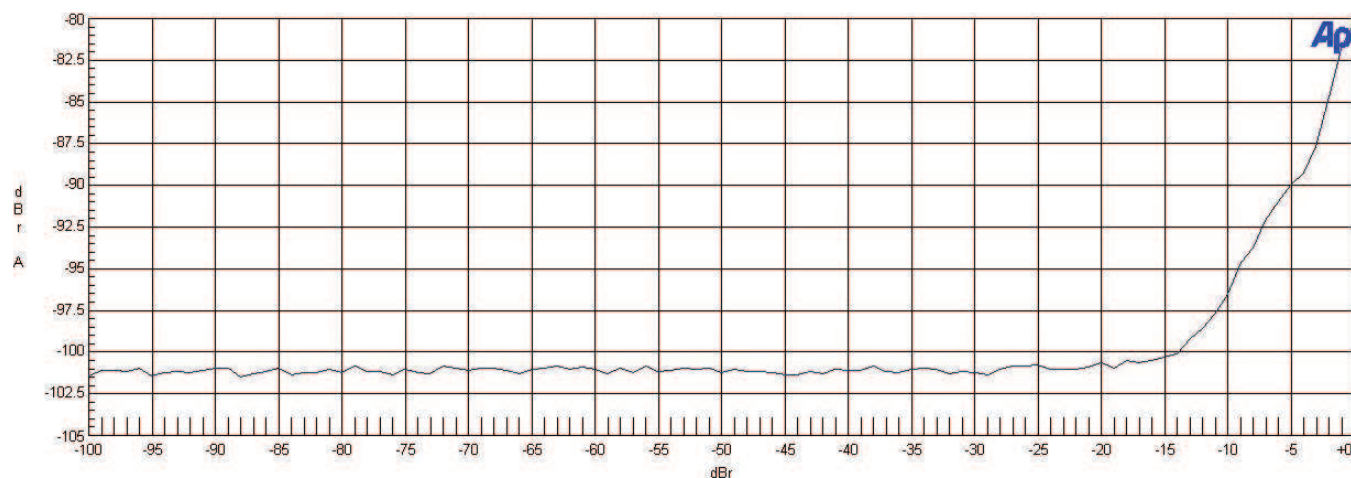
Figure 11-2. THD+N (ADC-DAC)
