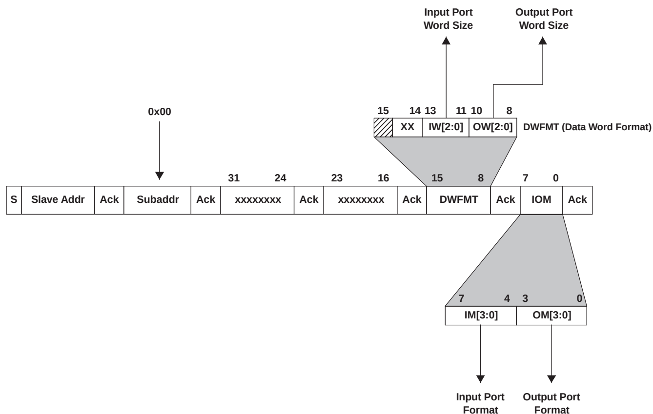
Figure 4-1. Serial Data Controls
