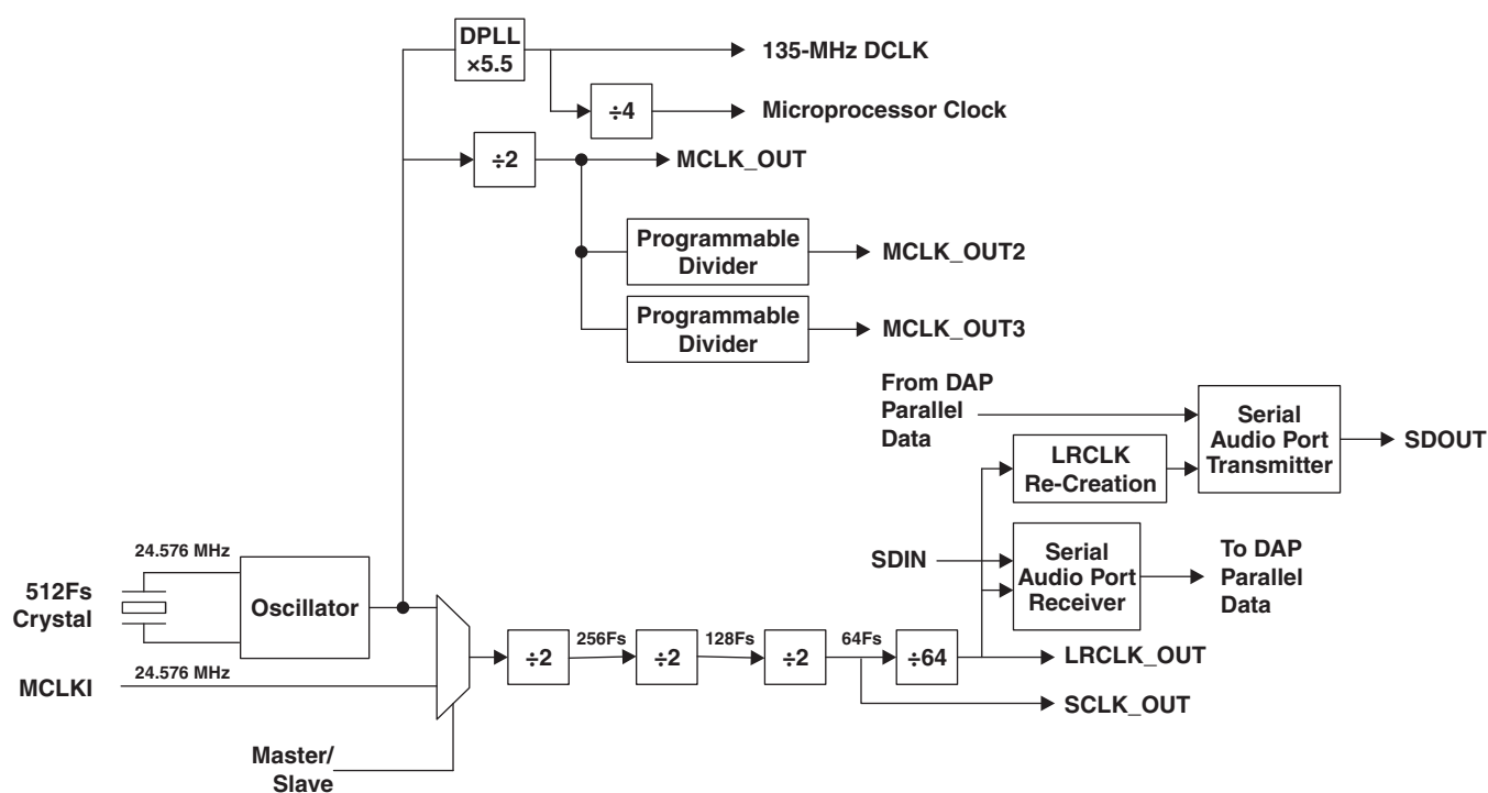
Figure 3-1. Clock Generation
