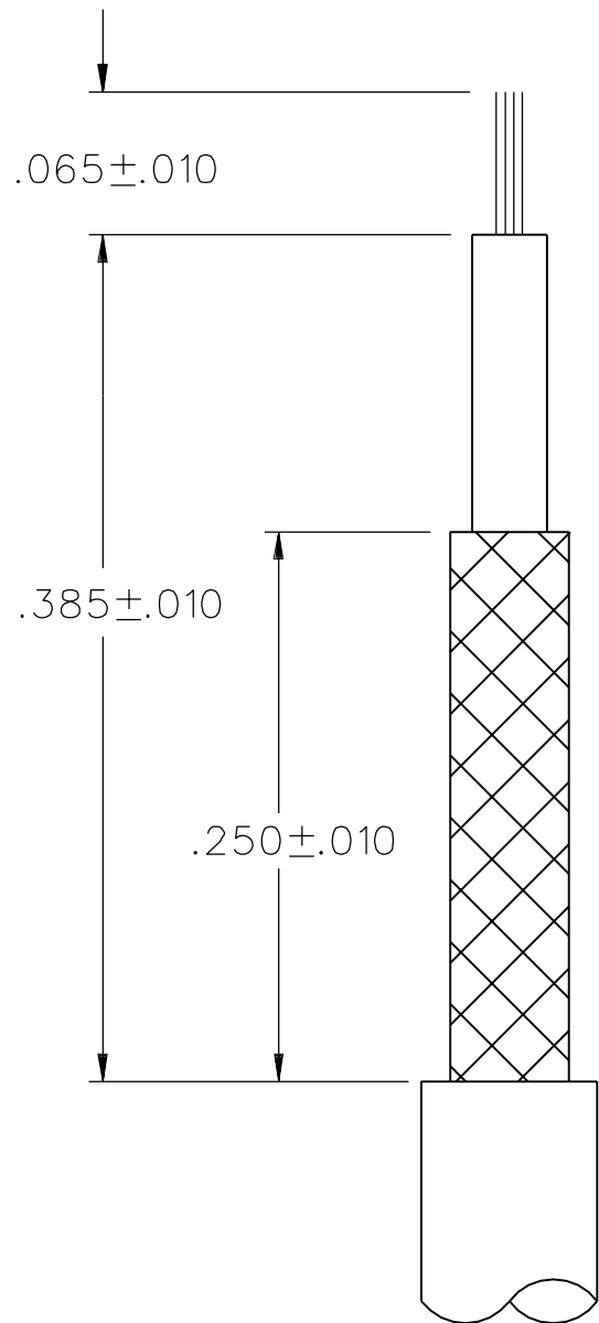
CABLE STRIP DIMENSIONS
