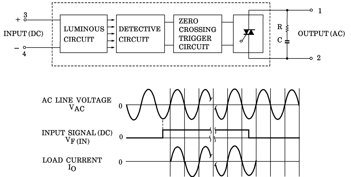
Fig.1 ZERO VOLTAGE SWITCHING WAVEFORM
