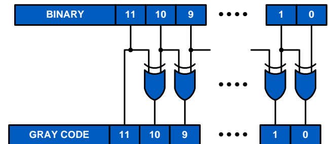
FIGURE 31. BINARY TO GRAY CODE CONVERSION
