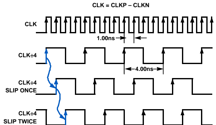
FIGURE 39. PHASE SLIP: CLK÷4 MODE, f_{\text{CLOCK}} = 1000\text{MHz}
