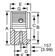
1/8" SHAFT=.126" (3.20) 1/4" SHAFT=.251" (6.38)
