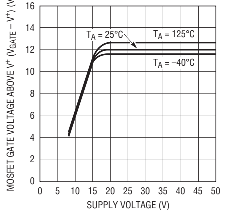
MOSFET Gate Voltage Above V^{+} ( V_{\text{GATE}} - V^{+} ) vs Supply Voltage
