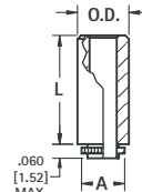
Clear Hole
