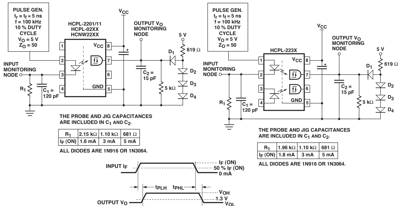
Figure 5. Circuit for t_{PLH} , t_{PHL} , t_r , t_f .
