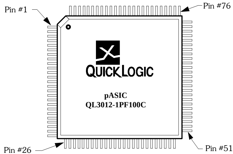
FIGURE 3. 100-Pin TQFP
