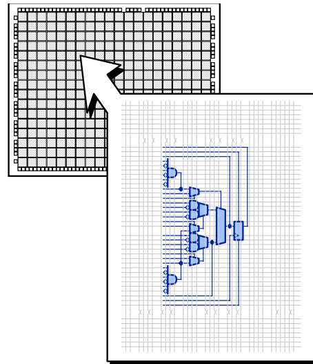
FIGURE 1. 320 Logic Cells
