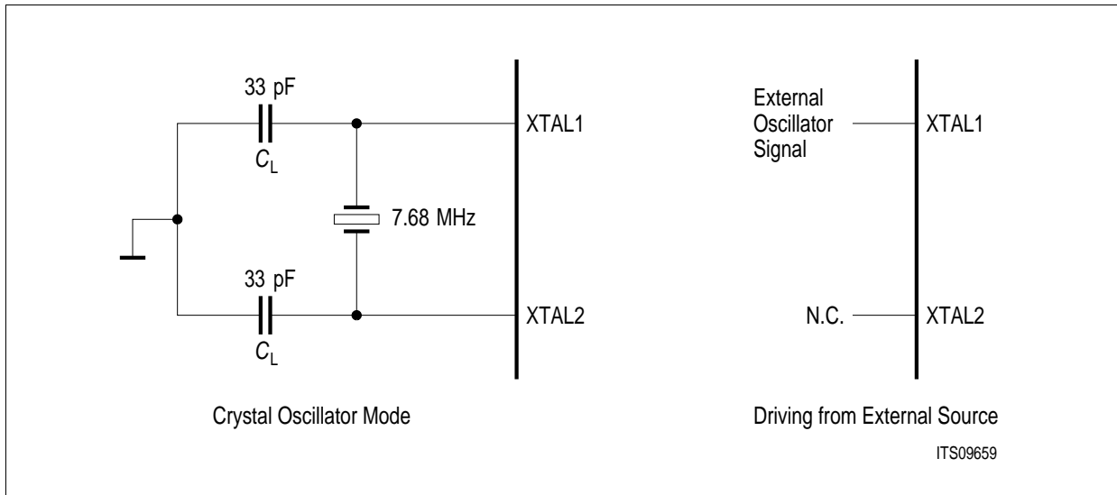
Figure 93 Oscillator Circuits
