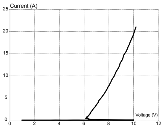
Figure 6. TLP characteristic
