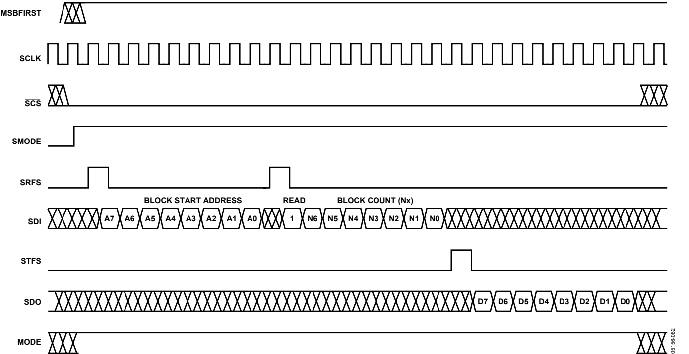
Figure 71. SPORT Read MSBFIRST = 1
