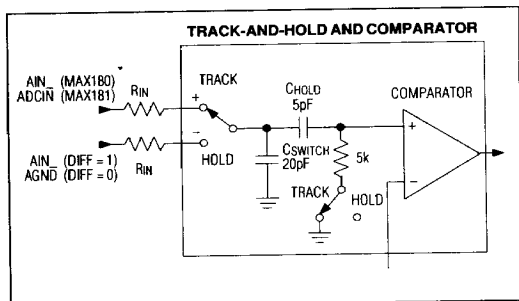
Figure 4. Equivalent Input Circuit
