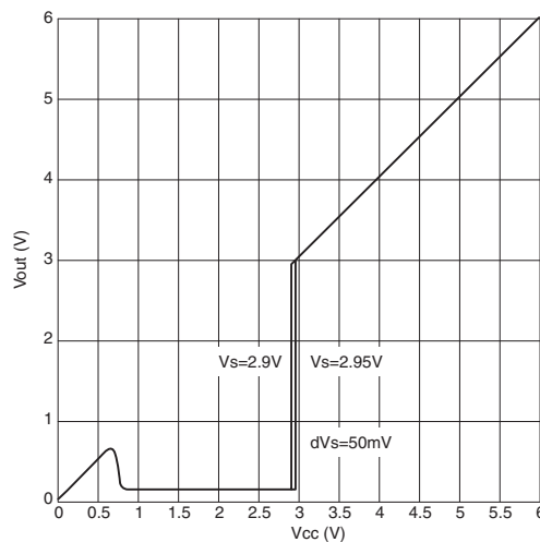
I/O characteristic
