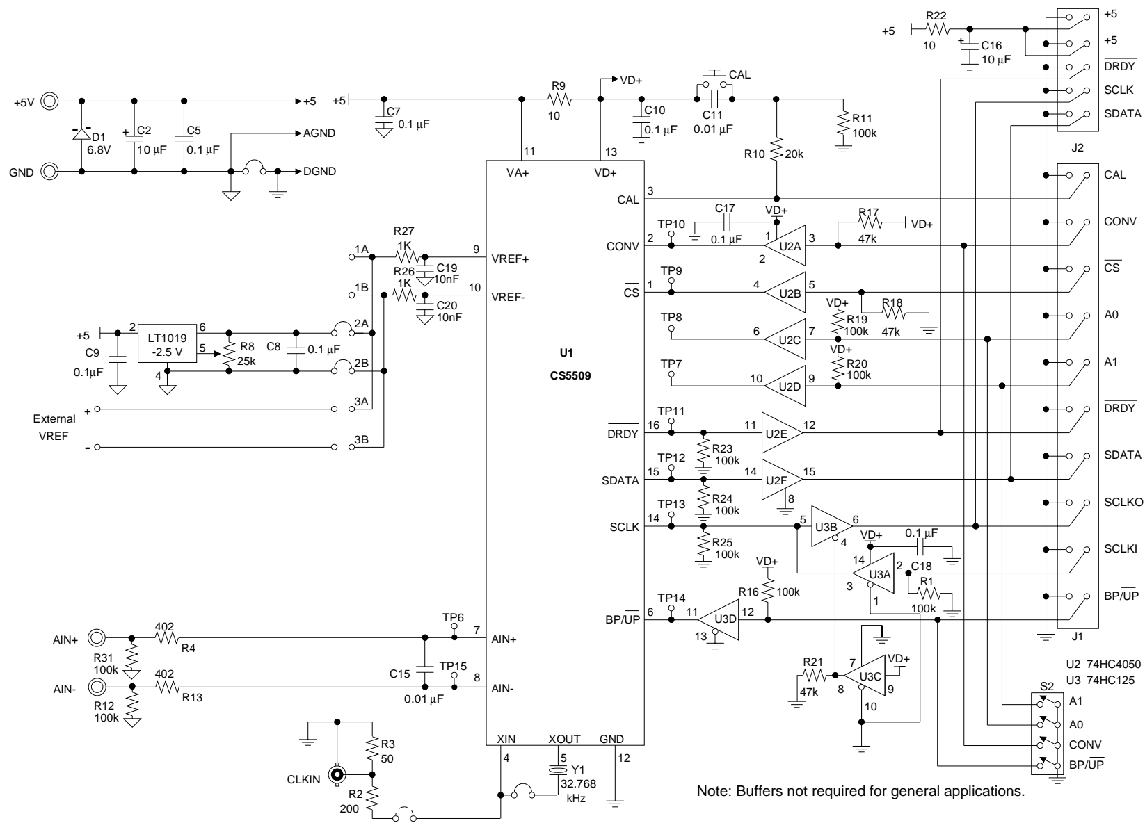
Figure 1. ADC Connections
