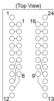
Figure 3. CAB5509 Adapter Board
