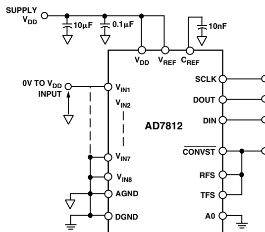
Figure 14. Evaluation Quick Setup
