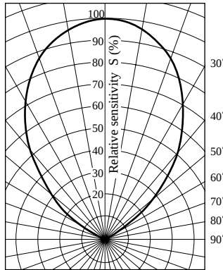
Directivity characteristics
