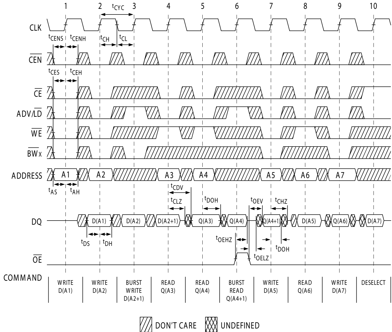
Figure 7. Read/Write Waveforms [37, 38, 39]
