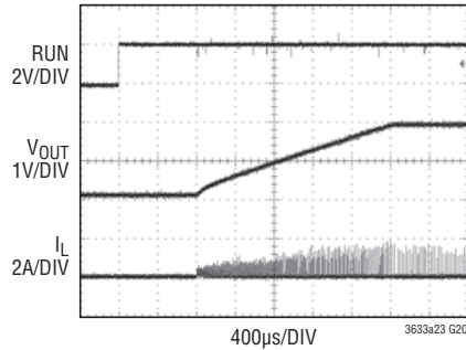
Start-Up (Burst Mode Operation)
