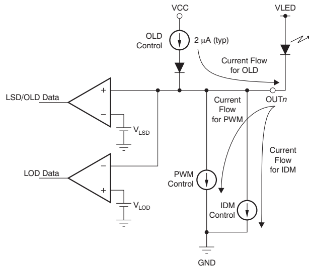
Figure 34. LOD/LSD/OLD/IDM Circuit
