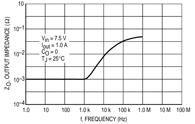
Figure 4. Output Impedance
