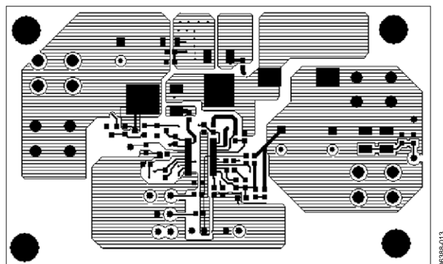
Figure 14. Top Layer
