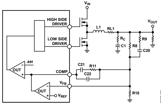
Figure 2. Control Loop
