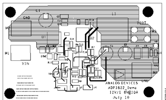
Figure 15. Bottom Layer
