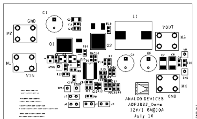
Figure 16. Silkscreen Top
