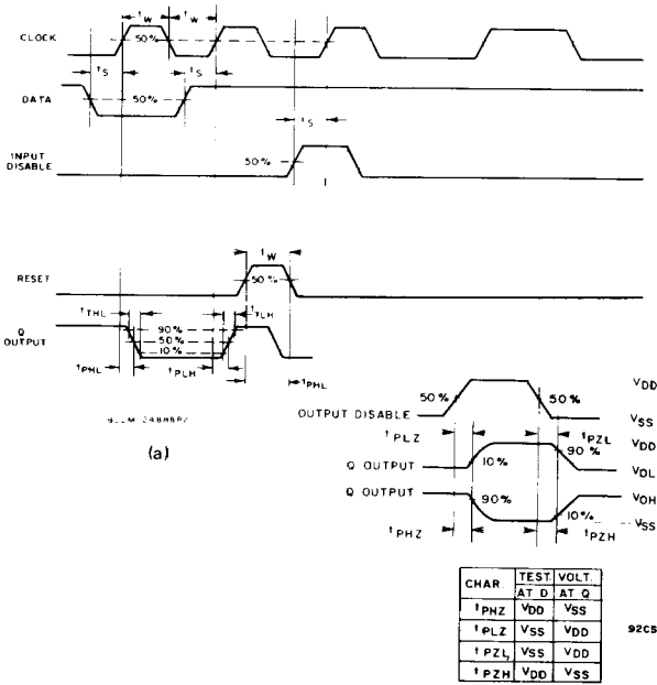
Fig. 5 — Functional waveforms for CD4076B.
