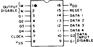
TERMINAL ASSIGNMENT
