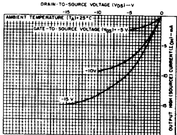
Fig. 4 — Minimum output high (source) current characteristics.
