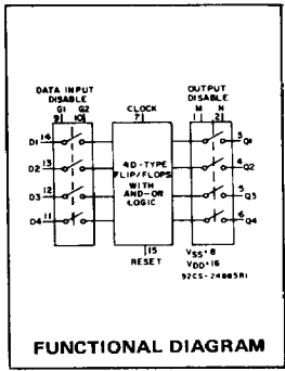
FUNCTIONAL DIAGRAM
