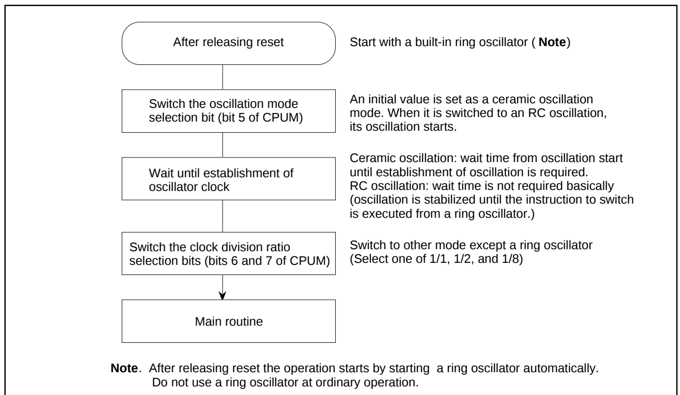
Fig. 10 Switching method of CPU mode register
