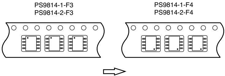
Taping Direction
